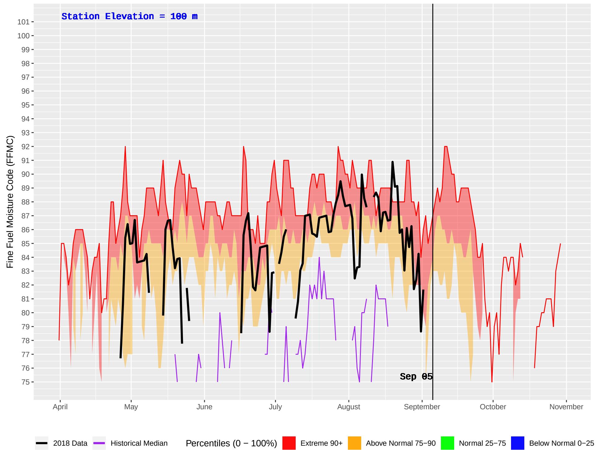
HONNA (93) : Historical (1986–2016) and Current (2018) Daily Fine Fuel Moisture Code (FFMC)
