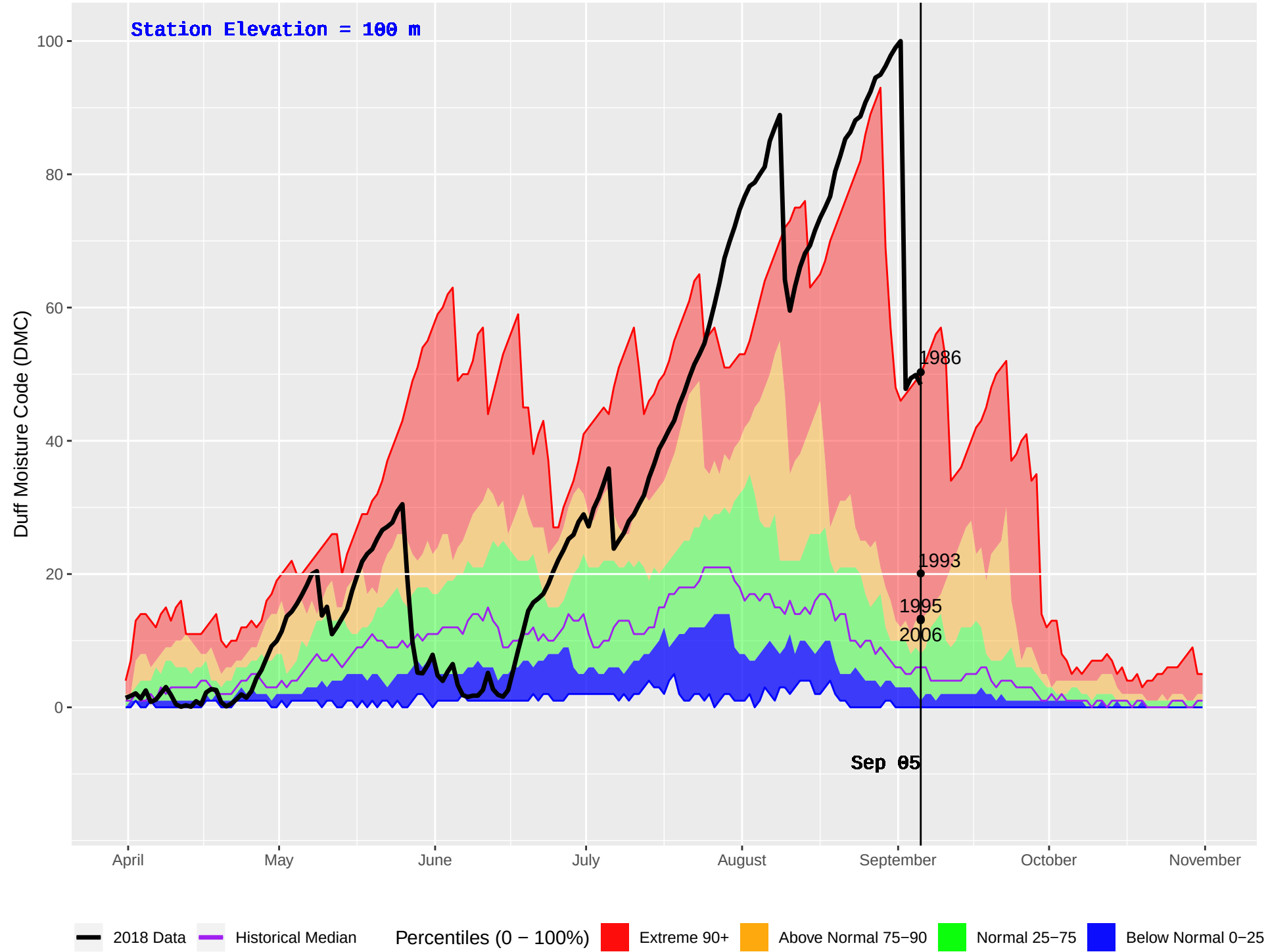
HONNA (93) : Historical (1986–2016) and Current (2018) Daily Duff Moisture Code (DMC)
