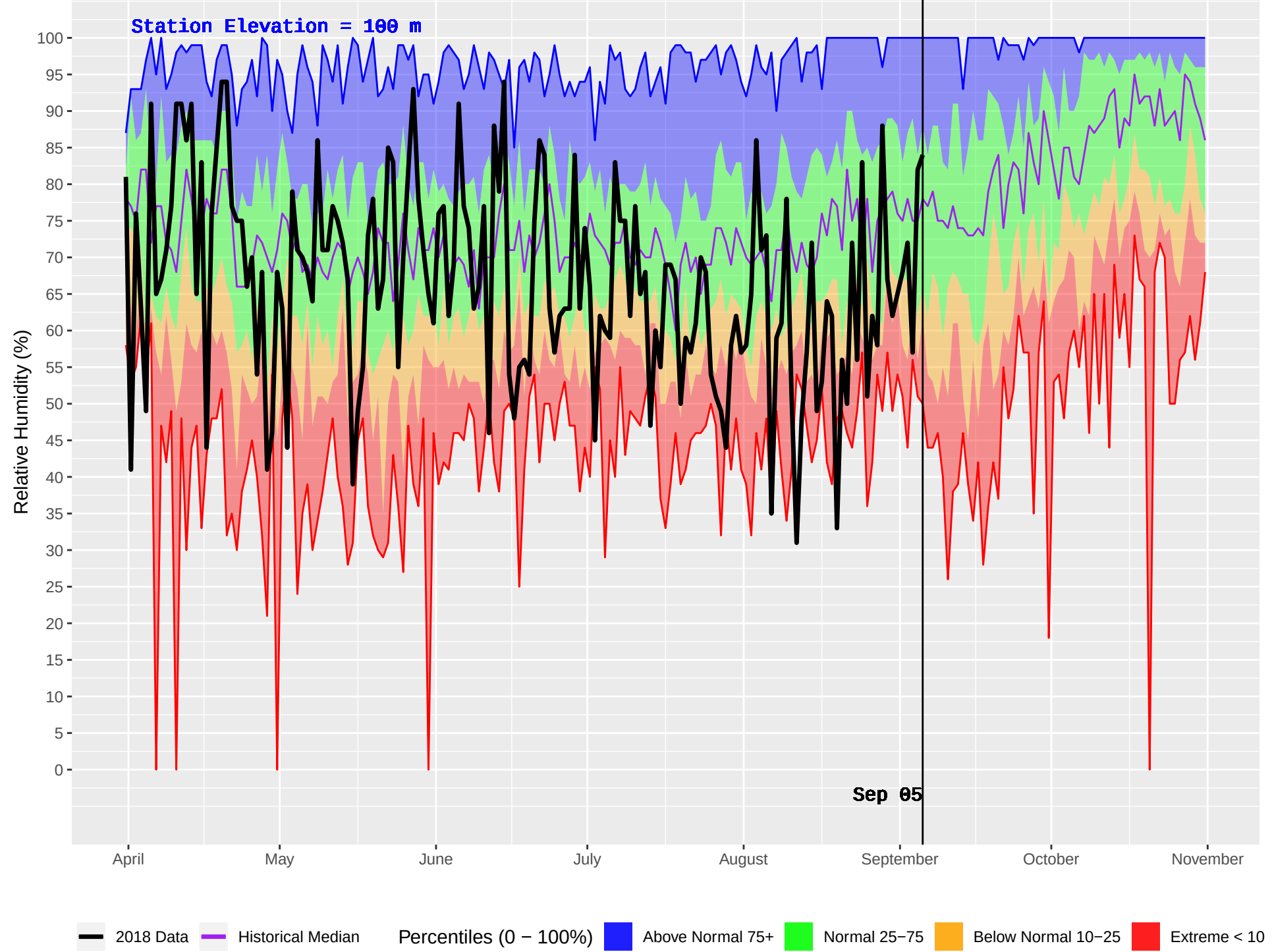
HONNA (93) : Historical (1986–2016) and Current (2018) Daily Relative Humidity
