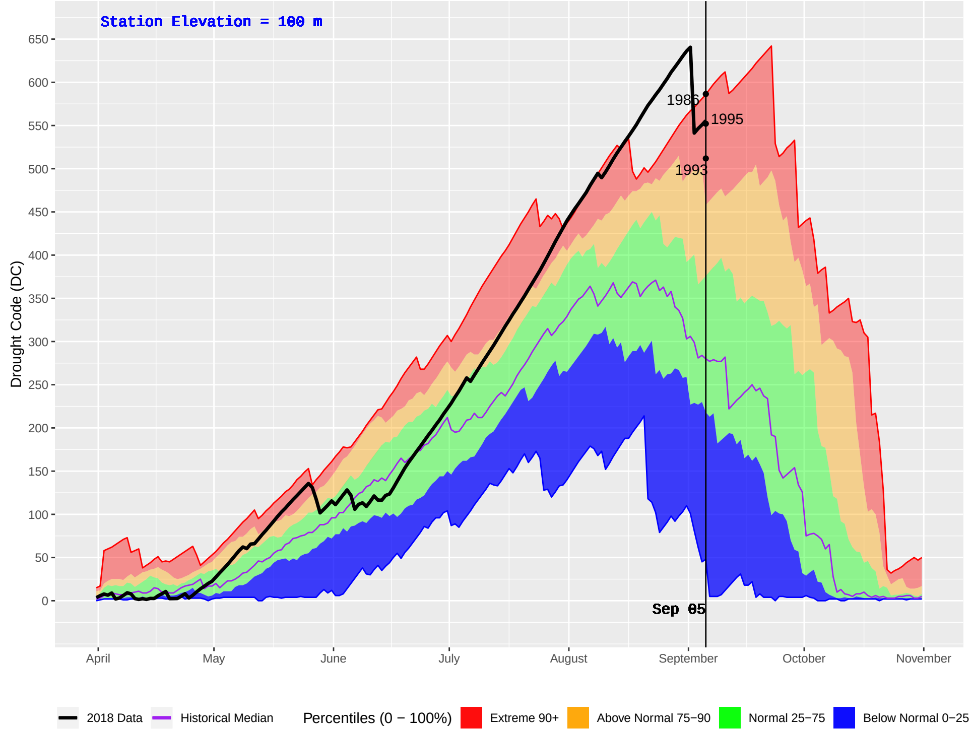
HONNA (93) : Historical (1986–2016) and Current (2018) Daily Drought Code (DC)
